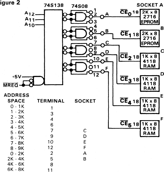
A satisfactory address-decoding solution for memories with two different capacities employs a decoder, an AND gate and appropriate jumpers or switches. This technique handles 1K- or 2K-word devices equally well.
