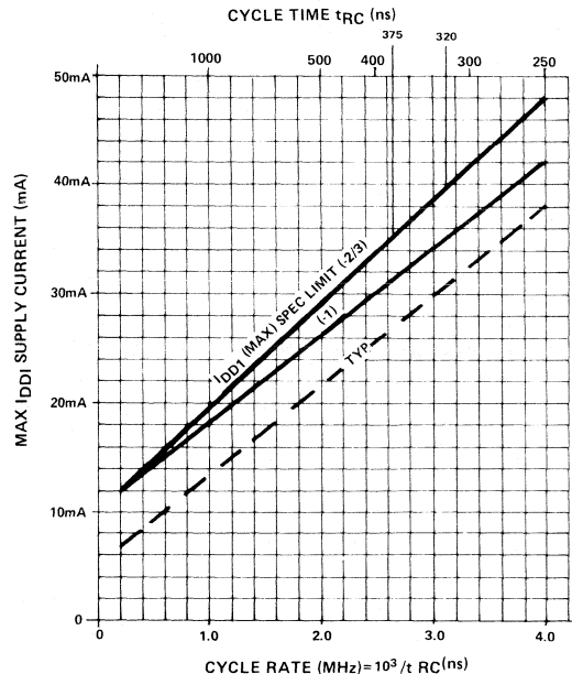
Fig. 4 Maximum I_{\text{DD1}} versus cycle rate for device operation at extended frequencies. I_{\text{DD1}} (max) curve is defined by the equation: I_{\text{DD1}} (max) mA = 10 + 9.4 x cycle rate (MHz) for -2/3 only I_{\text{DD1}} (max) mA = 10 + 8.0 x cycle rate (MHz) for -1 only
