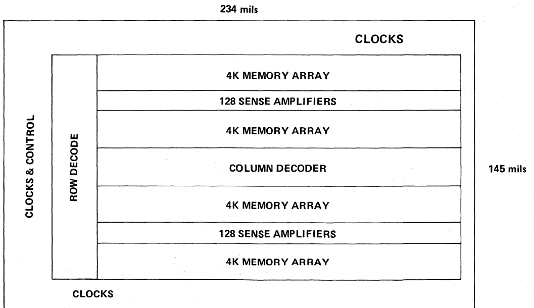
INTEL 2116
