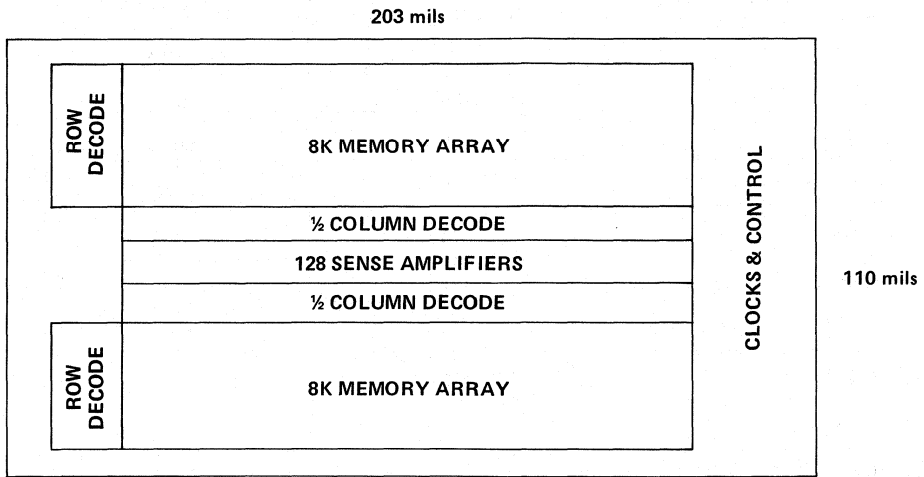
MOSTEK MK 4116
