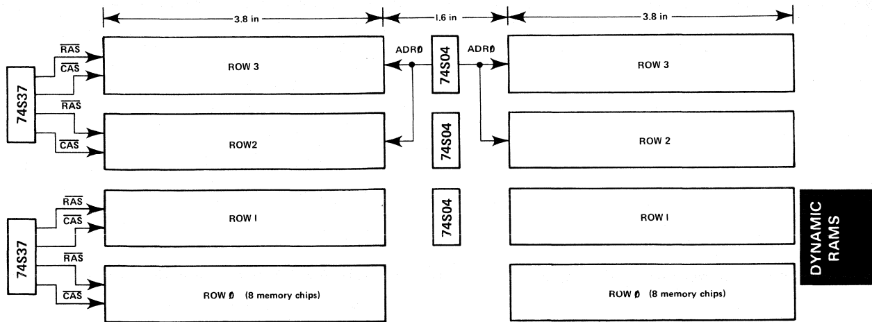
FIG. 16 TYPICAL PLACEMENT FOR DRIVERS WITHIN MEMORY MATRIX
