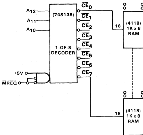
Address decoding for memories of identical capacity requires only a simple 1-of-8 decoder. A fixed 1K-word socket address space is shown.
