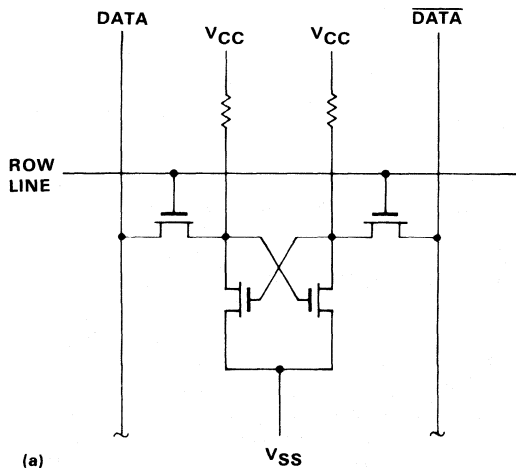
MK4104 CELL
