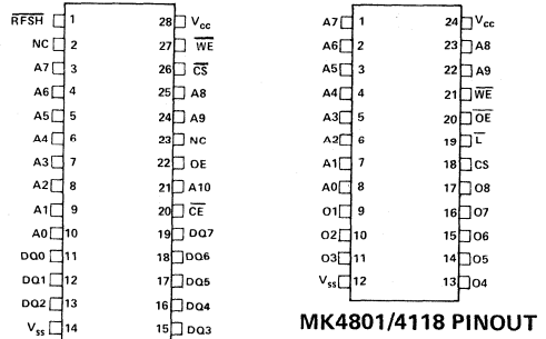
MK 4816 PINOUT
