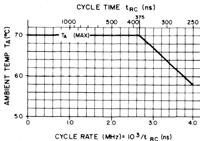
Fig. 1 Maximum ambient temperature versus cycle rate for extended frequency operation. T A (max) for operation at cycling rates greater than 2.66 MHz (t CYC < 375ns) is determined by T A (max) o C = 70 - 9.0 x (cycle rate MHz - 2.66) for -3.
