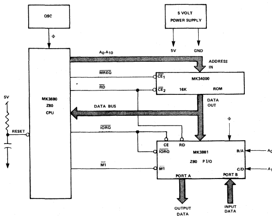
Typical microprocessor system utilizes CPU, P I/O, and 16K ROM.
