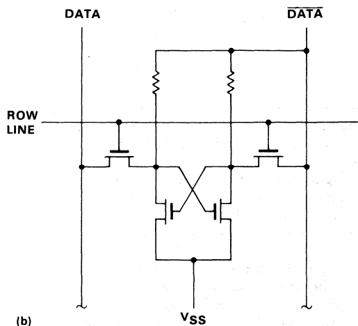
MK4118/4801 CELL
