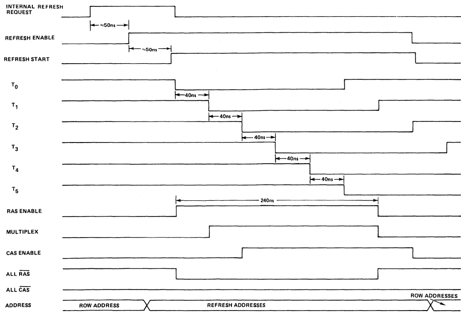
FIG. 11 INTERNAL REFRESH CYCLE TIMING
