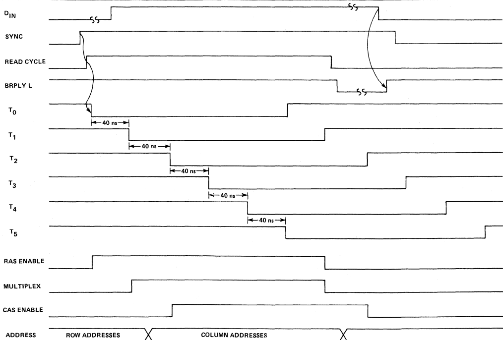
FIG. 9 READ CYCLE TIMING
