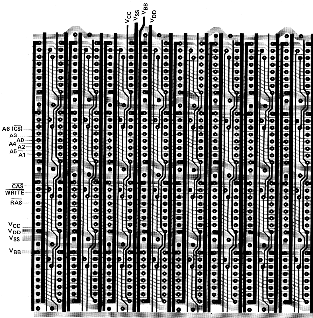
FIG. 15 SUGGESTED P.C. LAYOUT FOR MK4027 OR MK4116
