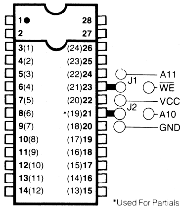
Figure 13 JUMPER LAYOUT
